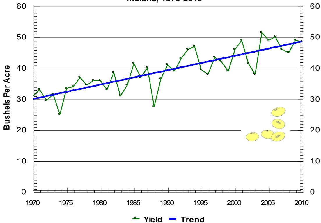
Soybean Yield Trend Indiana, 1970-2010
